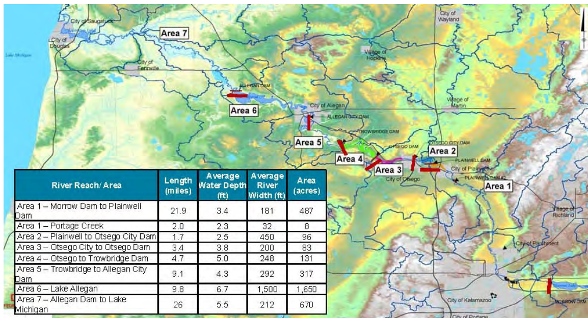
Figure 17. The seven areas of operable unit #5 of the Allied Paper, Inc./Portage Creek/Kalamazoo River Superfund site.
